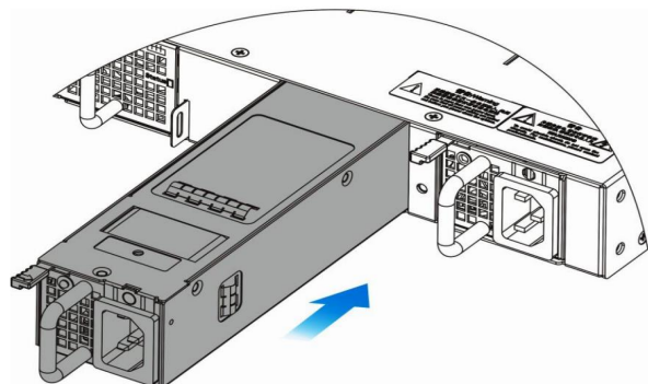
Figure 5: Installing PSM-C150WAC Power Module
