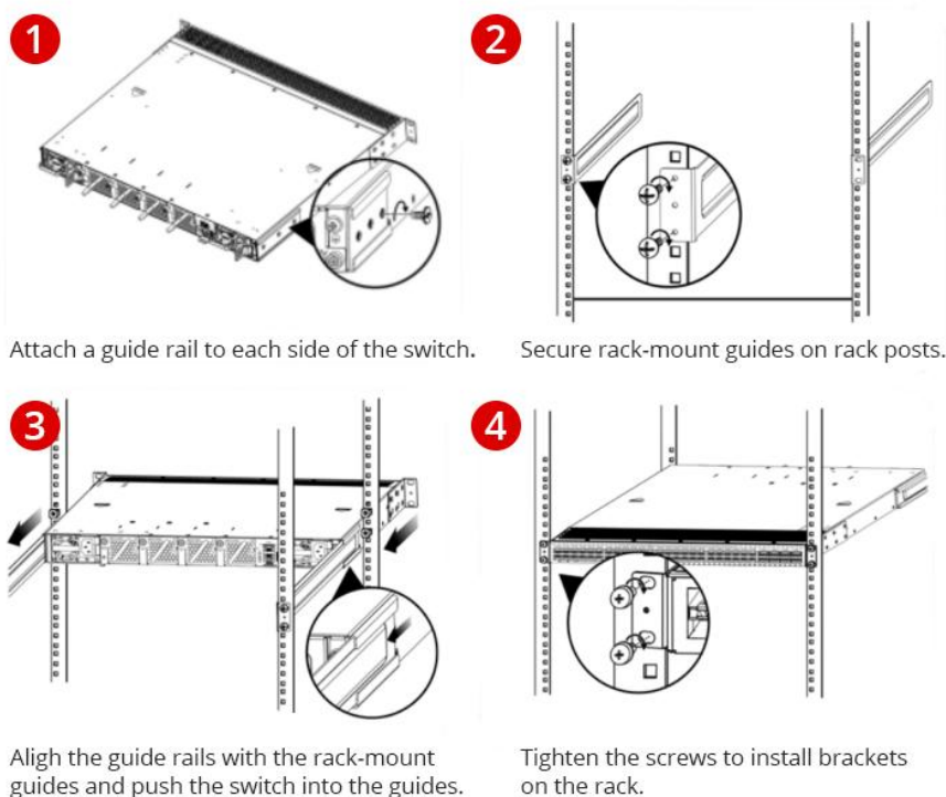
Figure 2: Mounting the Switch in a Rack
