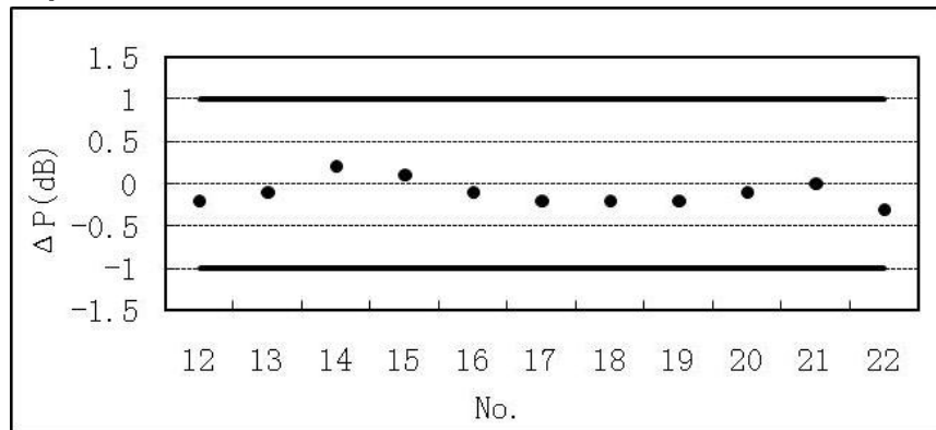
Figure 18: Optical Power Variation in Power Temperature Cycling Test
