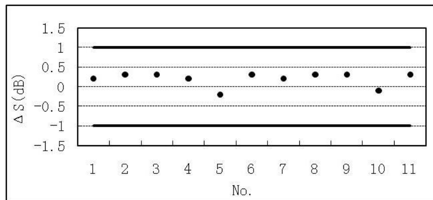
Figure 9: Receiver Sensitivity Variation in High Temperature Storage Test
