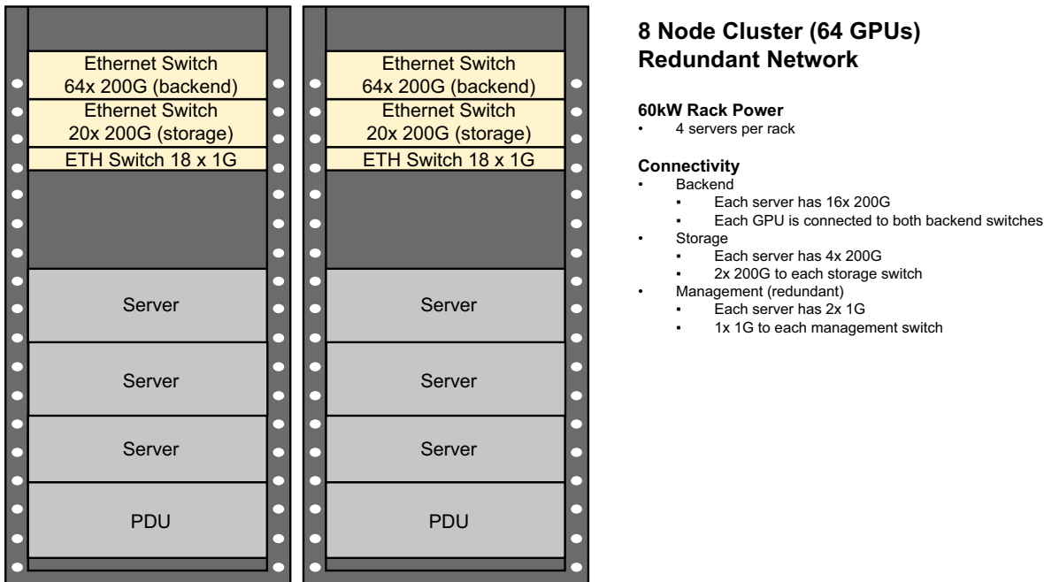
Figure 8: Rack View for 64 GPU Cluster, 60kW Rack Power – Redundant
