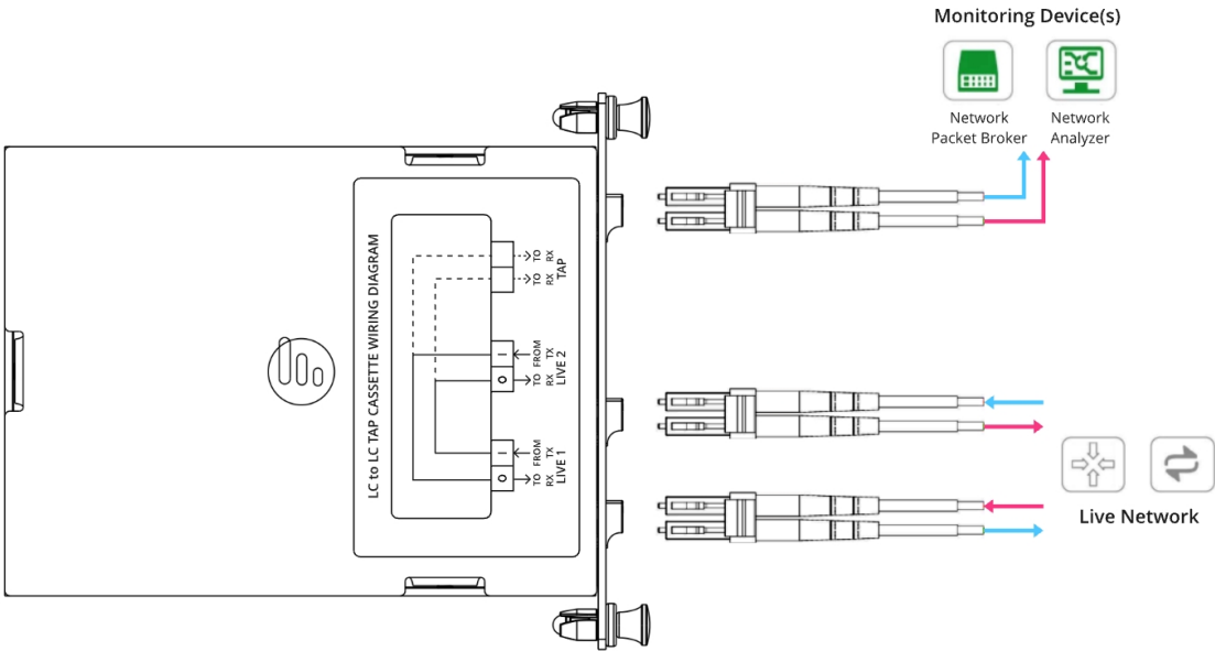
2 x LC Duplex Live Ports, LC Duplex TAP Ports
