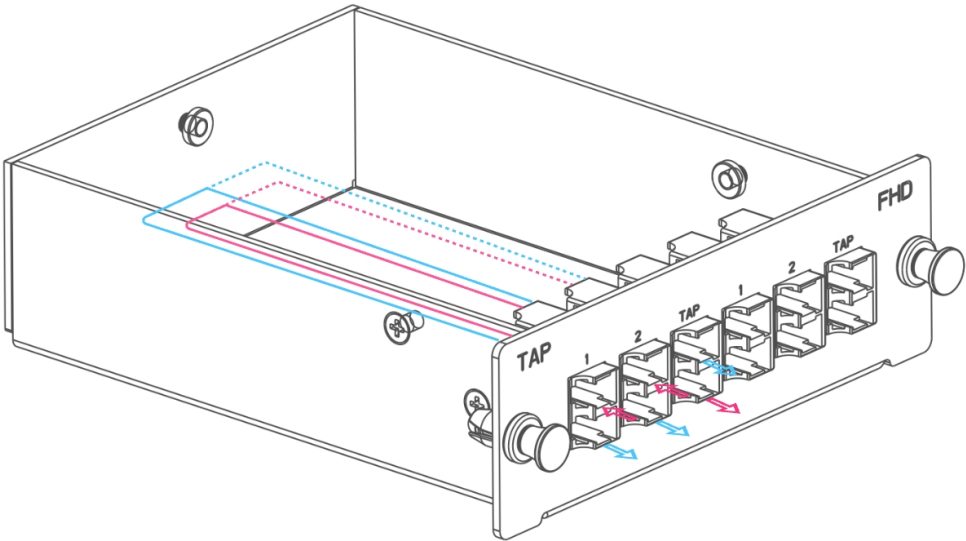
4 x LC Duplex Live Ports, 2 x LC Duplex TAP Ports
