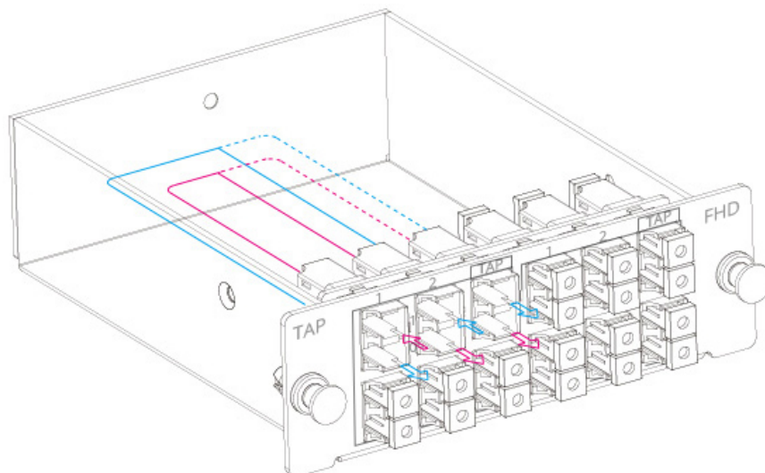
8 x LC Duplex Live Ports, 4 x LC Duplex TAP Ports
