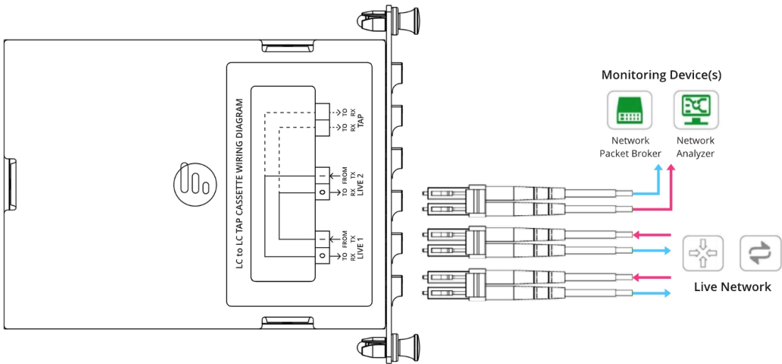
8 x LC Duplex Live Ports, 4 x LC Duplex TAP Ports / 4 x LC Duplex Live Ports, 2 x LC Duplex TAP Ports
