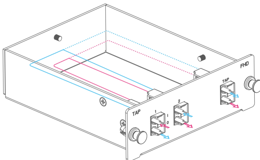
2 x LC Duplex Live Ports, LC Duplex TAP Ports
