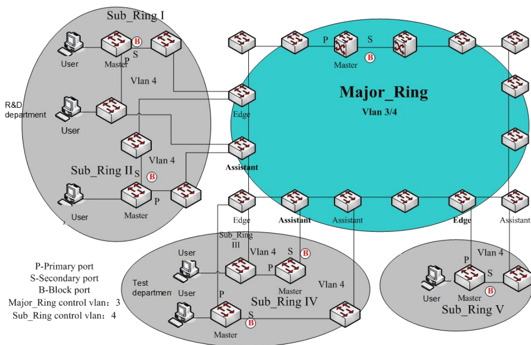
Figure 1 MEAPS Structure
