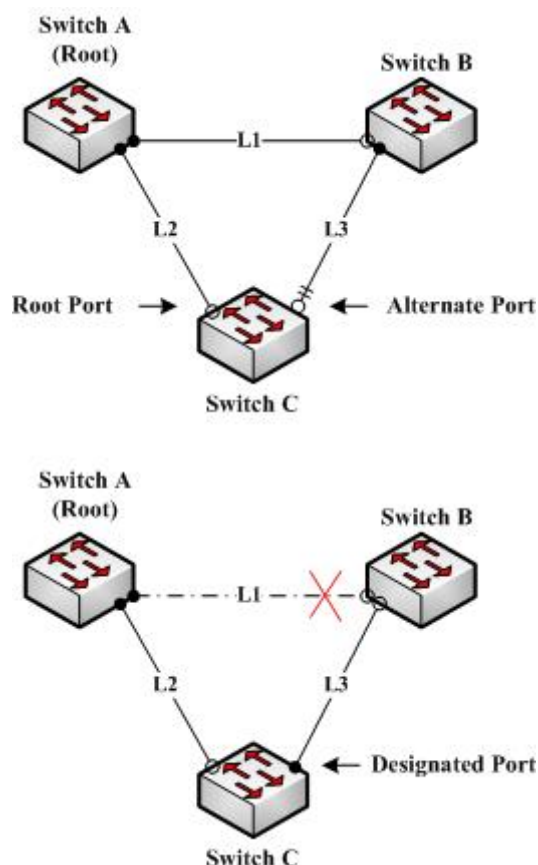
Figure 34-4 Backbone Fast
