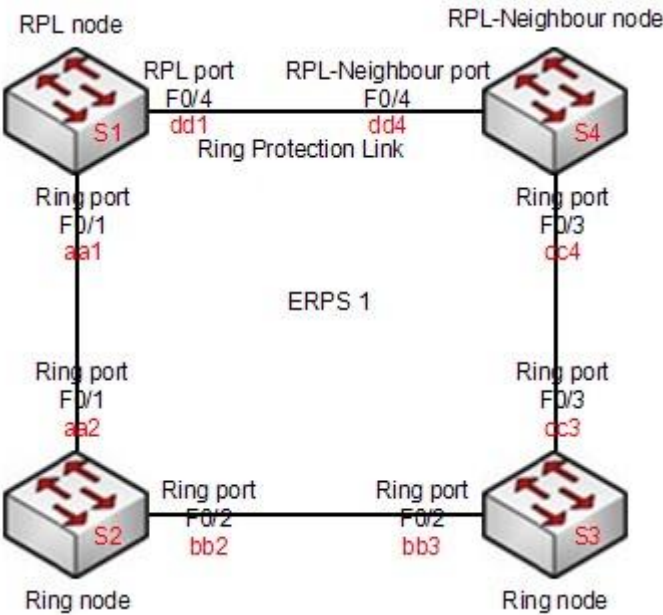
Figure 101. 1 ERPS Single Ring Configuration
