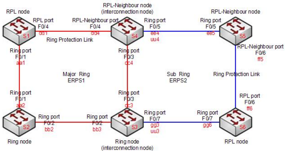
Figure 5.2 ERPS multi-ring configuration
