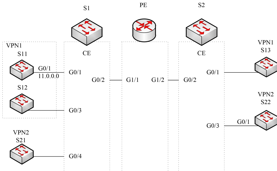
Figure 77.1 MCE configuration example
