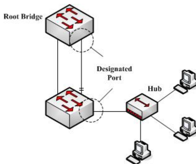
Figure 33-4 Designated port
