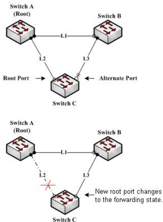
Figure 34-3 Uplink Fast
