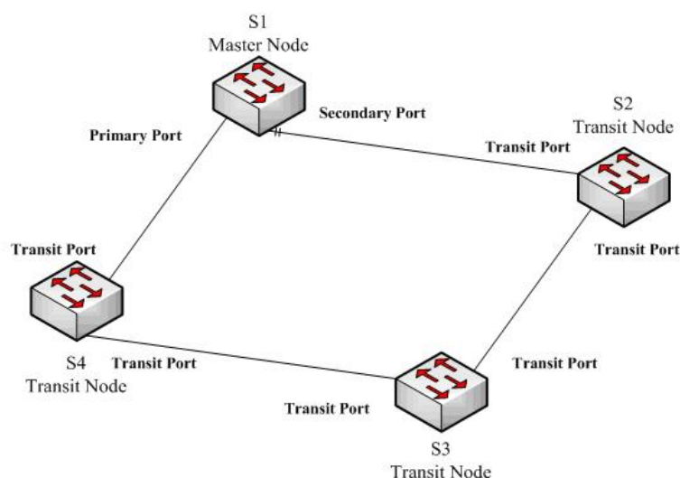
Figure 40.1 EAPS Ethernet ring
