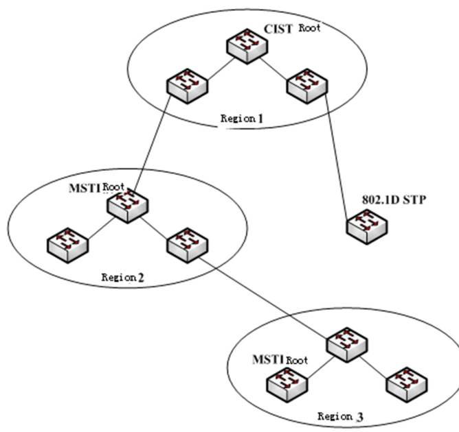
Figure 33-1 MSTP topology
