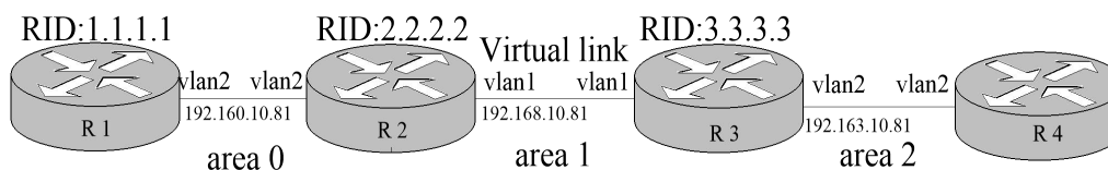
Figure 5- 2 Network Topology of the Example
