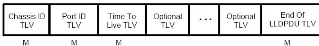
Figure 37-1 LLDP PDU Format
