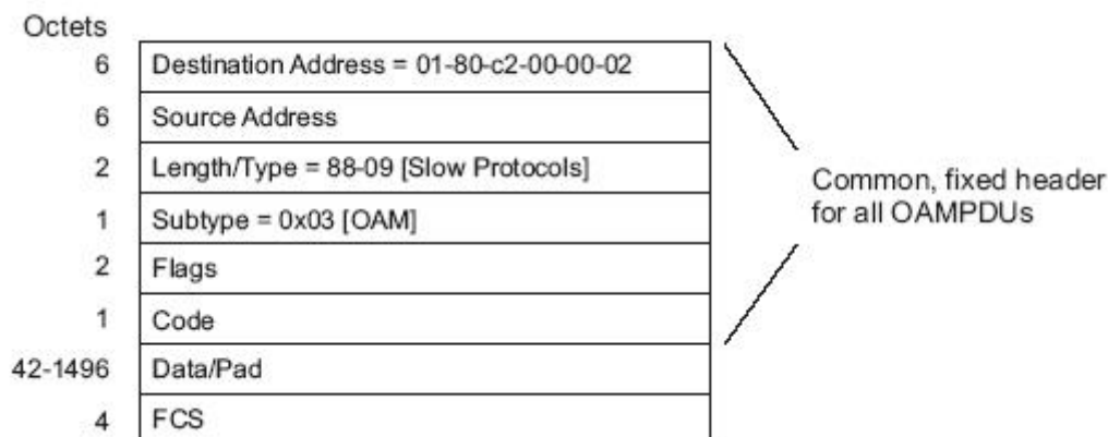
Figure 1 Components of the OAM packet
