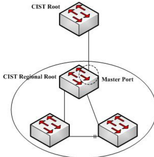
Figure 33-6 Master port
