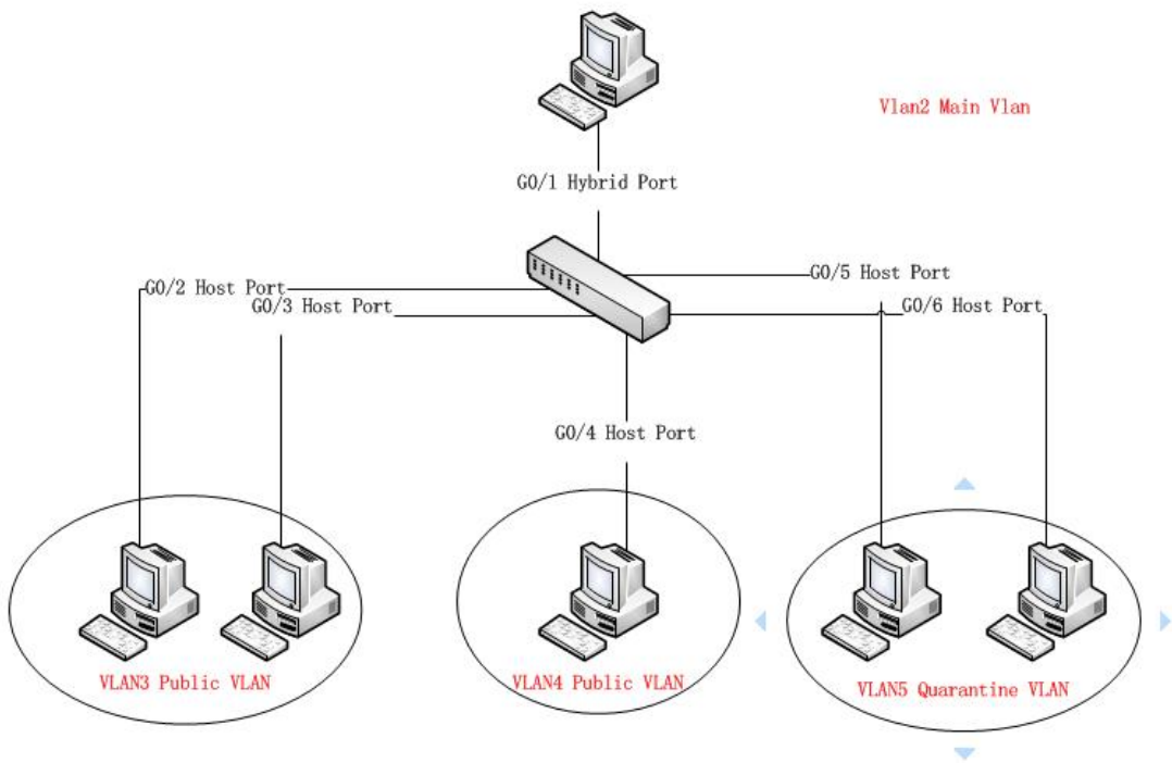
Figure 30-1: Typical Configuration of Private VLAN
