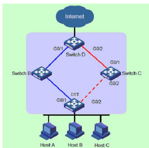
Diagram of BackupLink Address Aging Mechanism
